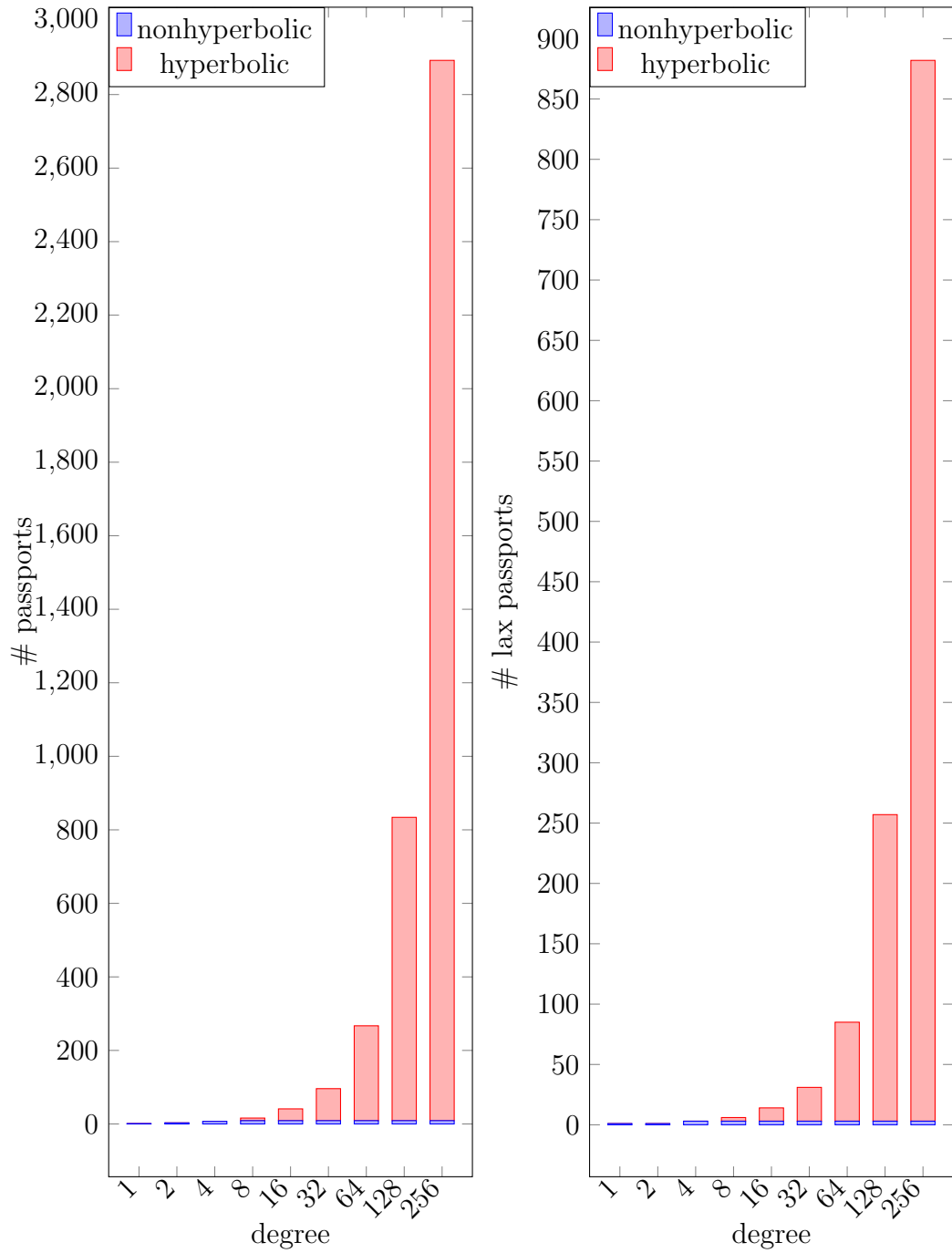
Figure 3.4.10: # nonhyperbolic and hyperbolic passports by degree (left), and # nonhyperbolic and hyperbolic lax passports by degree (right).
